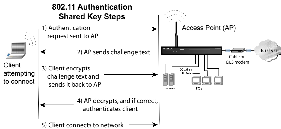
Figure 3-9: 802.11 shared key authentication
